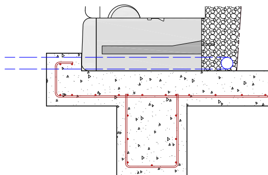
Figure 5D - Reinforced Concrete Leveling Pad
